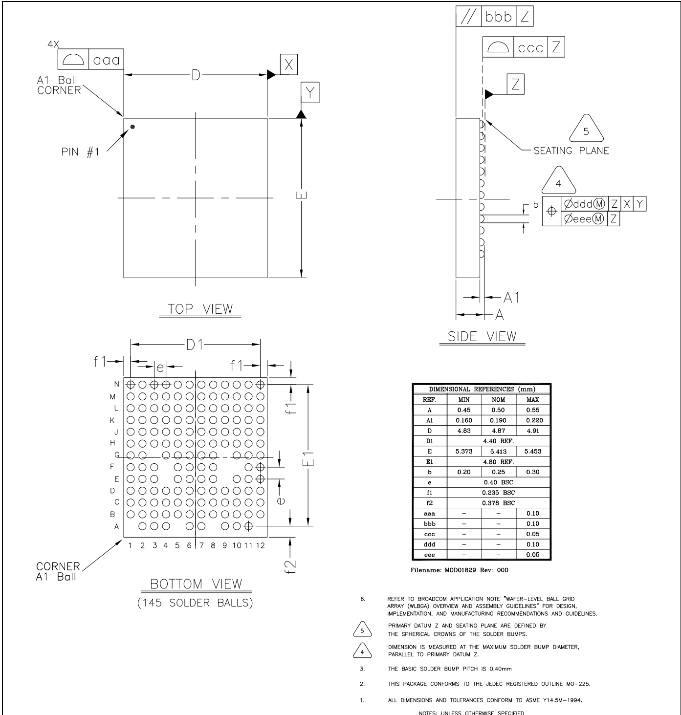
Figure 46. 145-Ball WLBGA Package Mechanical Information
